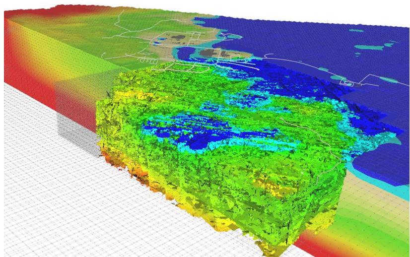
Site-scale DFN nested within a regional CPM model.
