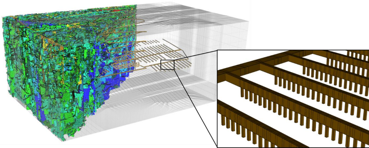
Geological disposal facility, with CPM tunnels embedded within a site-scale DFN model of fractured bedrocks.
